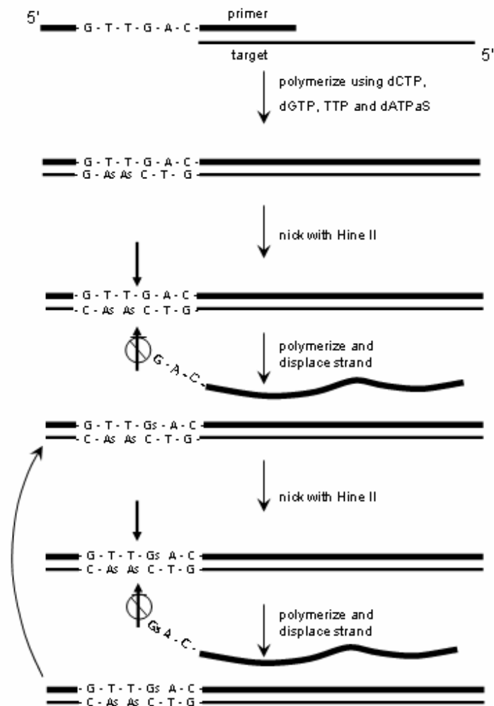
FIGURE 6.6 Strand-displacement amplification (SDA).
