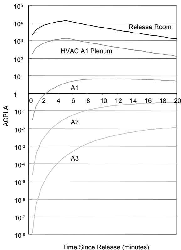
FIGURE 10.4 Early time anthrax concentrations, with no HVAC response.
