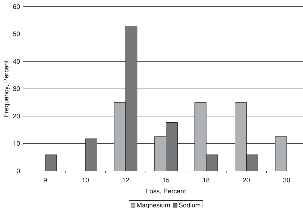
Figure 28. Frequency distribution of sulfate soundness specifications.
