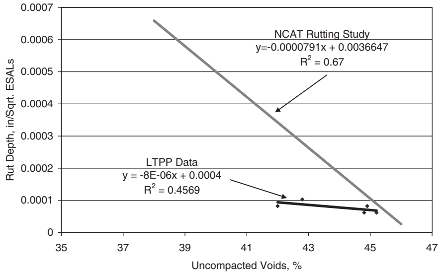
Figure 29. Uncompacted voids versus rut depth normalized by traffic (10).
