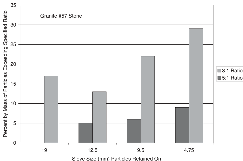
Figure 24. Example of shape variation with particle size.
