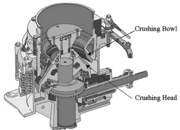
Figure 20. Cutaway view of Symons cone crusher (156, originally from Nordberg, Inc., Milwaukee, WI).
